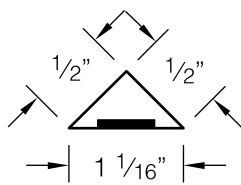
1/2" reveal strip
