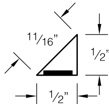
1/2" chamfer strip
