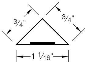
3/4" reveal strip
