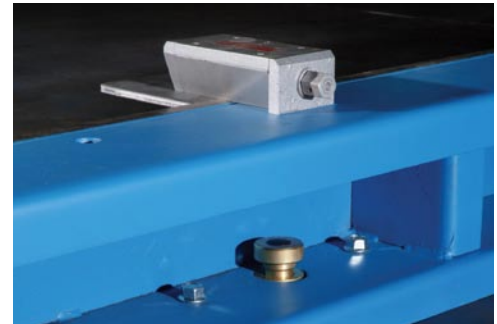
Side rail anchored to casting table with button magnets. On/Off magnet used to hold welding plate in place.
